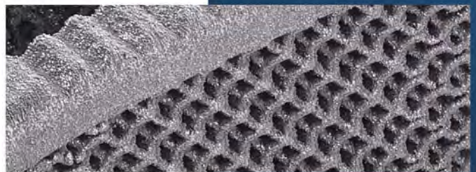
Implantable interbody cage – Titanium; Direct Metal Printed.
